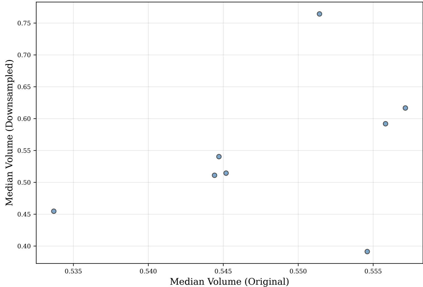
Median Volume: Original vs Downsampled sigma: (0.02, 0.4) | volume: (0.03, 0.9)
